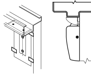
Top Latch & 108 Strike
