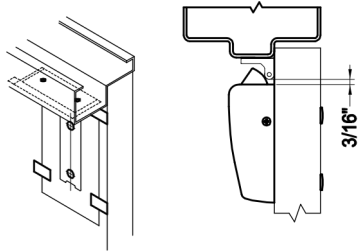
Top Latch & 106/106Z Strike
